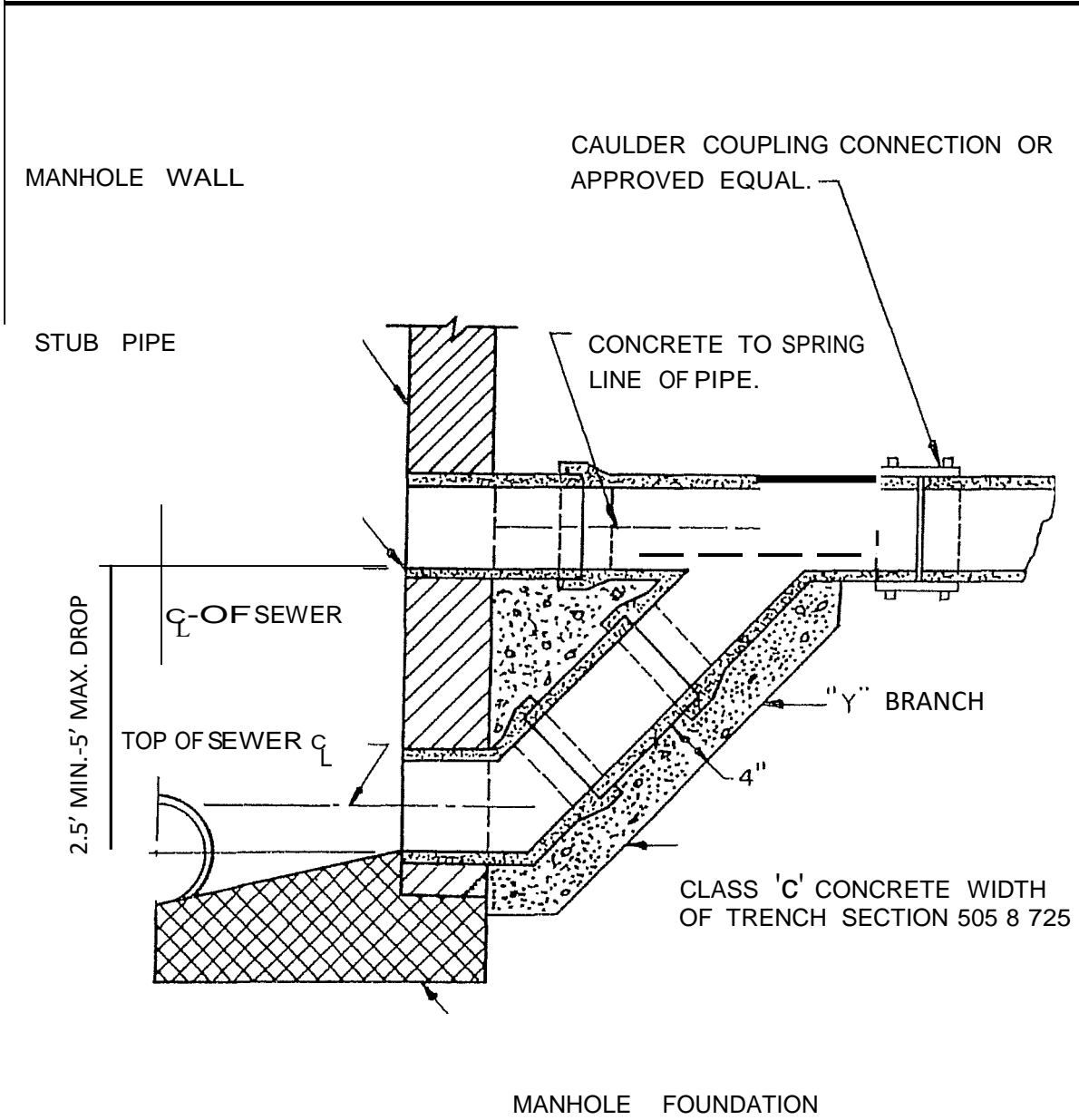
TYPE A 2.5' TO 5' DROP
