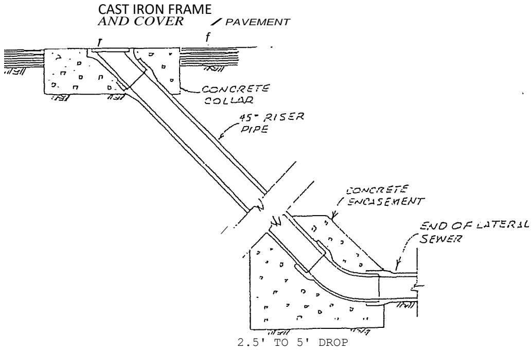
SLANT LATERAL CLEANOUT
