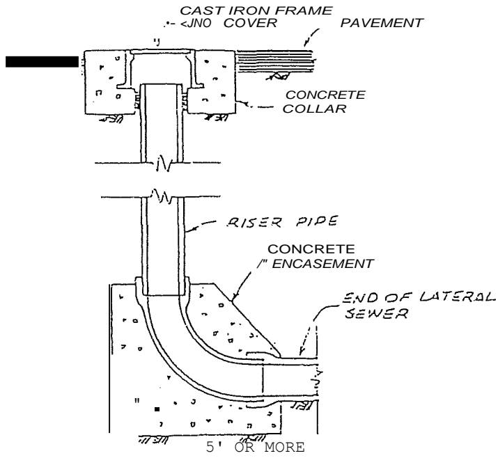
Vertical lateral cleanout
